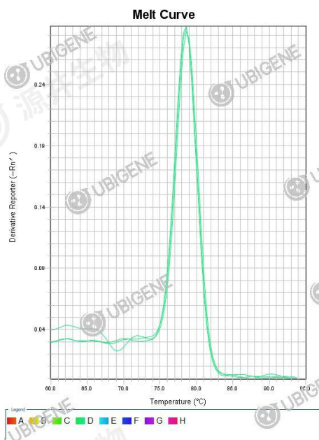
HepG2_Ctrl(Puro)+ hASNS-1 melt curve
