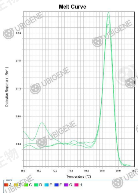
ASNS Stable Expression Cell Line (Hep G2)+ \beta -h_actin melt curve
