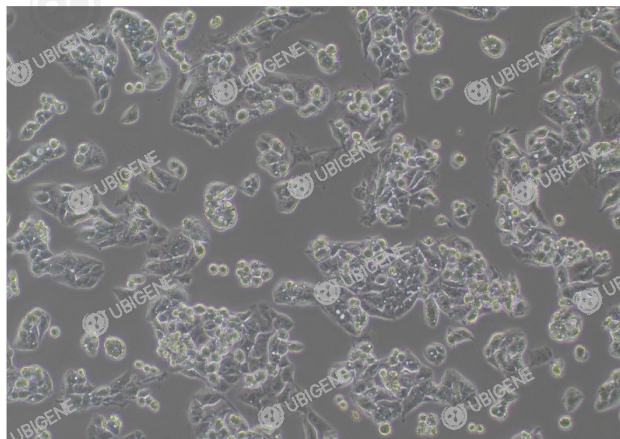
ASNS Stable Expression Cell Line (Hep G2)-100X
