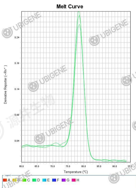
ASNS Stable Expression Cell Line (Hep G2)+ hASNS-1 melt curve
